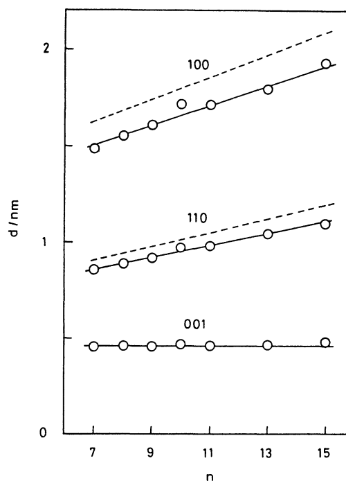
Fig. 1. Plots of spacings measured in M 1 phases against the number of carbon atoms in the alkyl group for compounds 2 . Broken lines indicate the corresponding spacings of compounds 1 .
